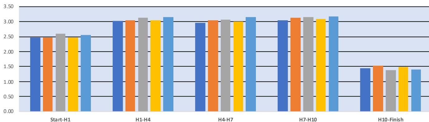
Hurdle Phases
